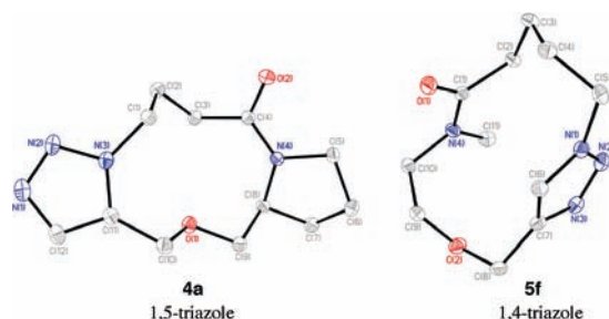
Figure 1. X-ray crystal structures of representative macrocyclic triazoles ( 4a and 5f ).
